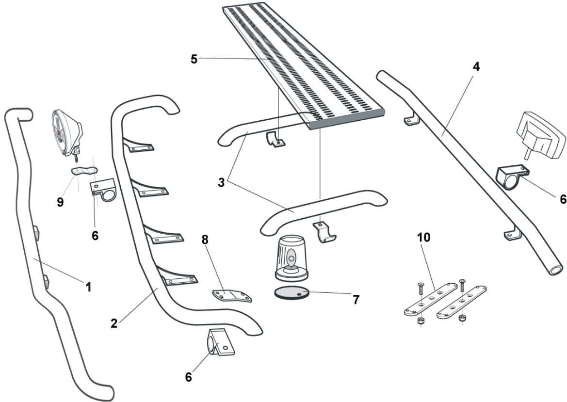
Front Top-Bar, with mounting kit
